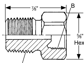
Female Inverted Flare x Male NPT
