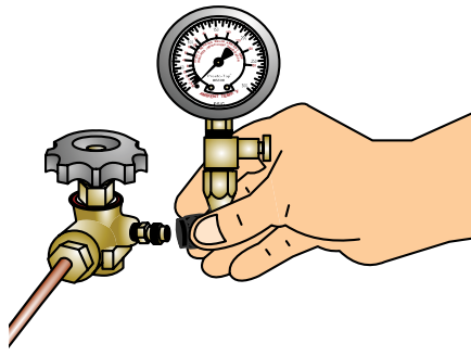
2 Attach 300 LB Gauge to pressure fitting. Perform System Leak Test Per NFPA 58 - Your Company Policy.
