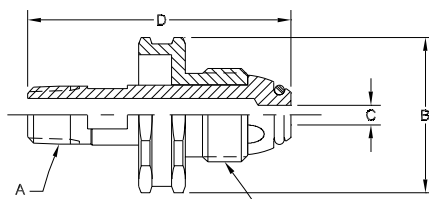
970AW 970HT Soft Nose POL w/Handwheel
