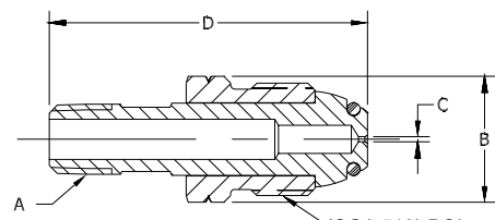
970S Soft Nose POL w/60 DMS Orifice
